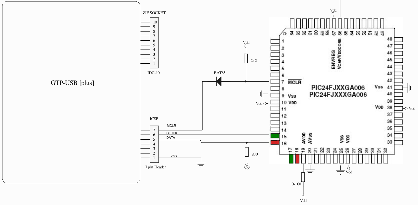
PIC24F ICSP Connection of example
